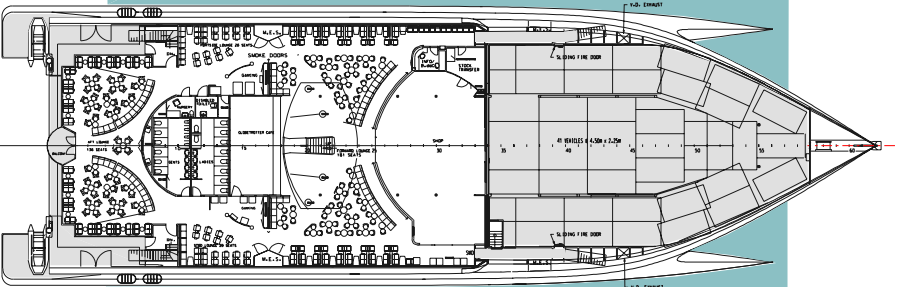
TIER 2 PLAN
