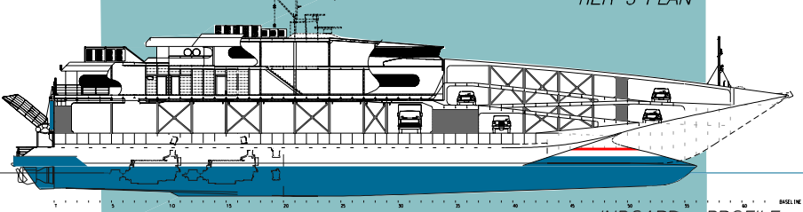
INBOARD PROFILE
