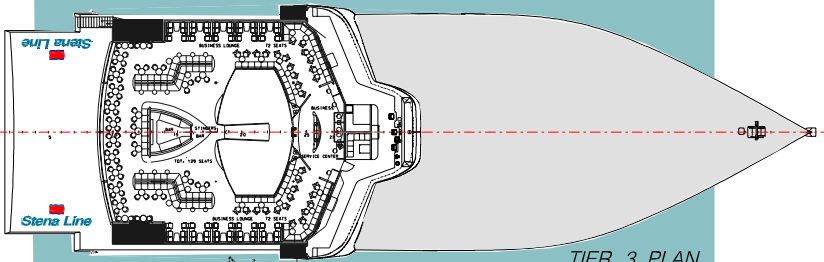
TIER 3 PLAN
